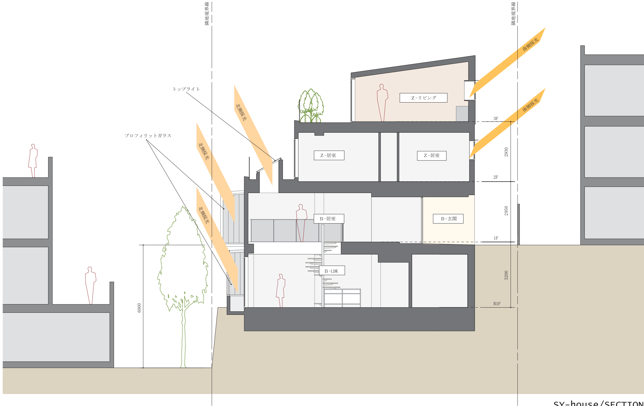
SY-house/SECTION
